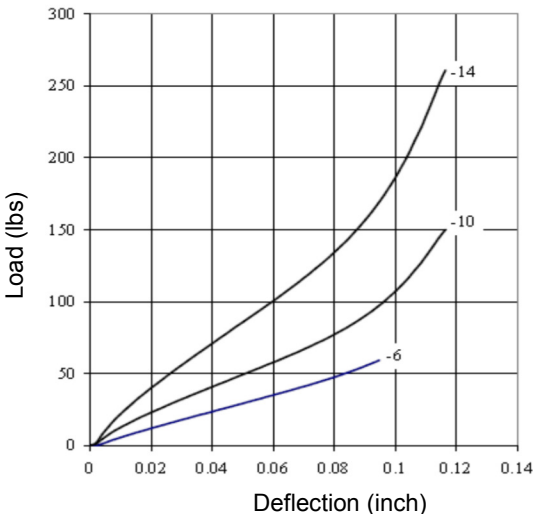
Typical Load vs. Deflection
