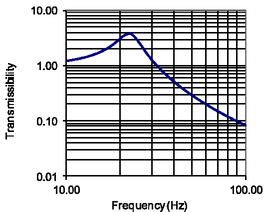
Transmissibility vs. Frequency
