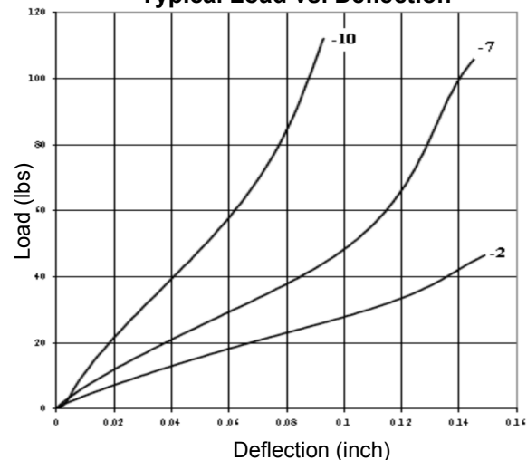
Typical Load vs. Deflection
